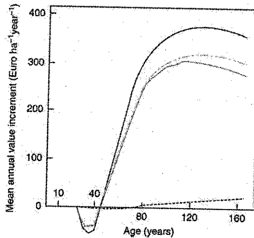
FIG. 7. Scenario analysis with SILVA2.2 on stand level. Current annual volume growth (top) and mean annual value increment (bottom) in pure stands of Norway spruce compared with mixed stands of Norway spruce and European beech (Pretzsch, 2001, pp. 258–261).
