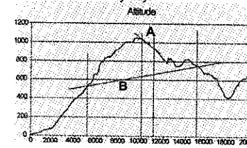
Figure 5. Graph showing problems with determining slope using different scales. A. shows slope across 1 km (between 10 and 11 km from coast) of -10%. B. shows slope over 10 km (between 5 and 15 km from coast) of +2.5%.
