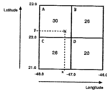
Figure 1. A 4-cell grid with a representative point (x, y) .
