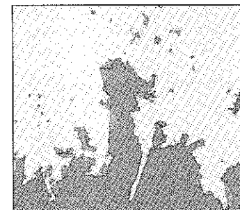
Figure 2. Example of coastlines at two different scales: 1:5,000,000 and 1:500,000.
