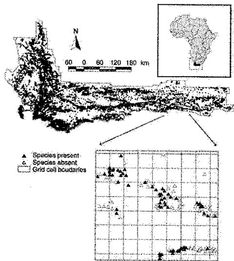
FIG. 1. The Cape Floristic Region with Protea Atlas Project sample points overlaid. The thumbnail shows the region's location on the African continent. The pull-out box displays, for a small (12 × 13 km) part of the region, the grid cells used for modeling and sample locations scattered across these grid cells, including both sample locations at which Protea mundii was observed (solid triangles) and the "null sites" at which it was not (open triangles).
