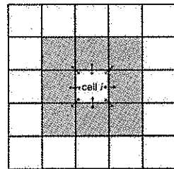
FIG. 3. Diagram of the grid cell neighborhood used in the conditional autoregressive (CAR) models employed in Models 2 and 4.
